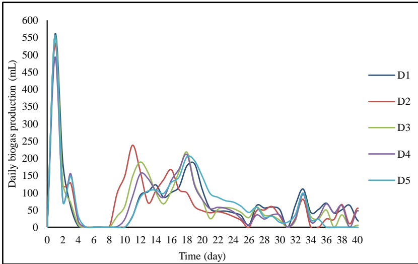
Figure 6. Daily biogas production versus time
